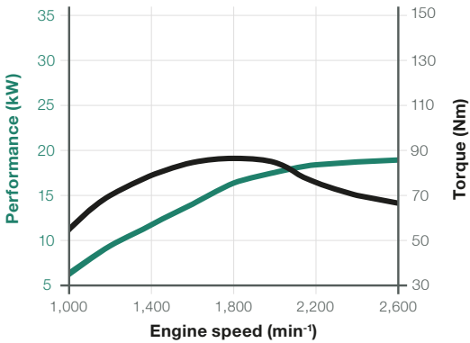
Performance curve of Yanmar 8TNV80FT; 18.4 kW; stage V (standard)
