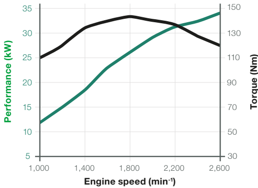
Performance curve of Yanmar 3TNV86CHT; 33.3 kW; stage V (option)
