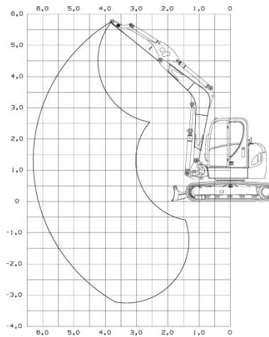
Fig. 2: Lifting force tables 75Z3 –long dipper stick
