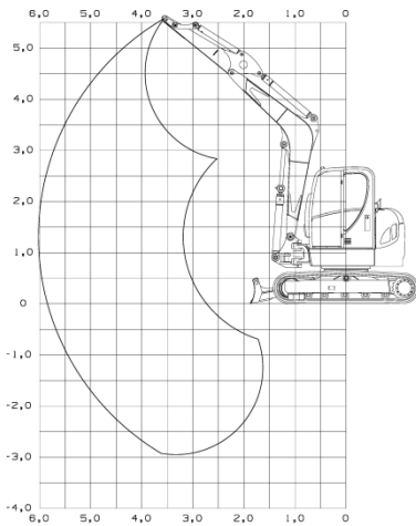
Fig. 1: Lifting force tables 75Z3
